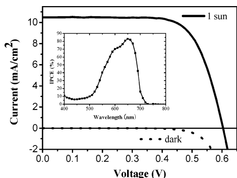
Figure 2. Photocurrent action spectrum (inset) and current–voltage characteristics of the squaraine dye obtained with a nanocrystalline TiO 2 film supported onto a conducting glass sheet and derivatized with a monolayer of squaraine dyes in the presence of chenodeoxycholic acid. A sandwich-type cell configuration was used to measure the spectrum.
